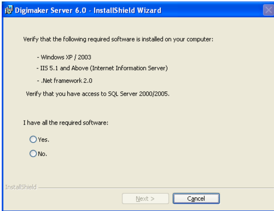
Figure 2: Required Software
